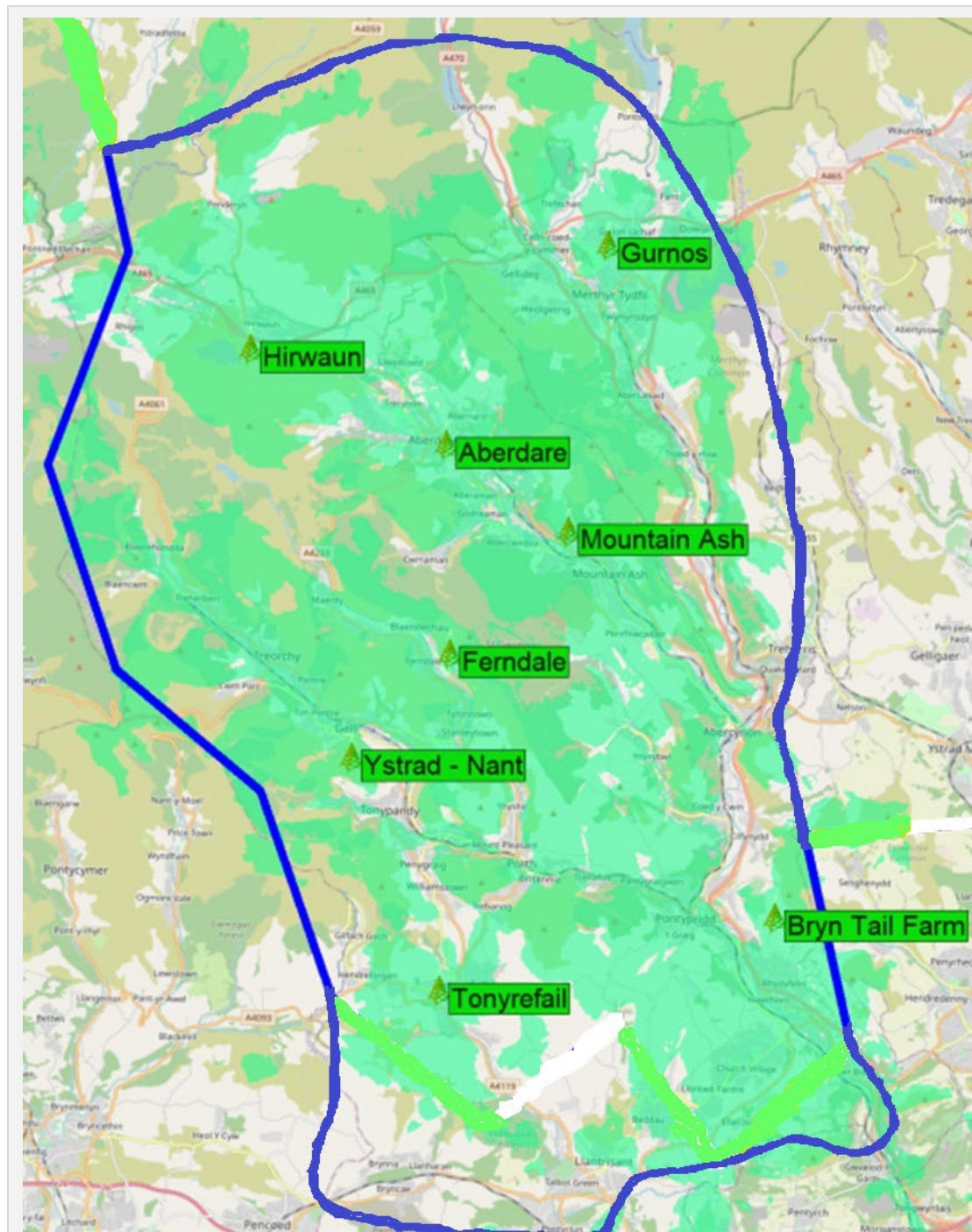
GTFM Valleys Multiplex - predicted coverage at 63 dBμV/m field strength from 8 transmitter sites with reference to the advertised licence area outlined in blue.
