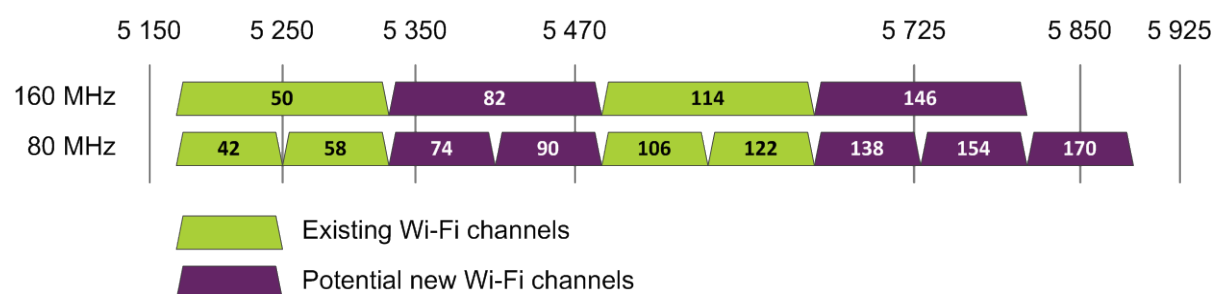
Figure 4.3 Example channelisation for Wi-Fi at 5 GHz
