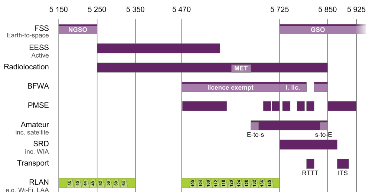
Figure A5.1: Existing RLAN and incumbent services and applications in 5150-5925 MHz in the UK/EU
