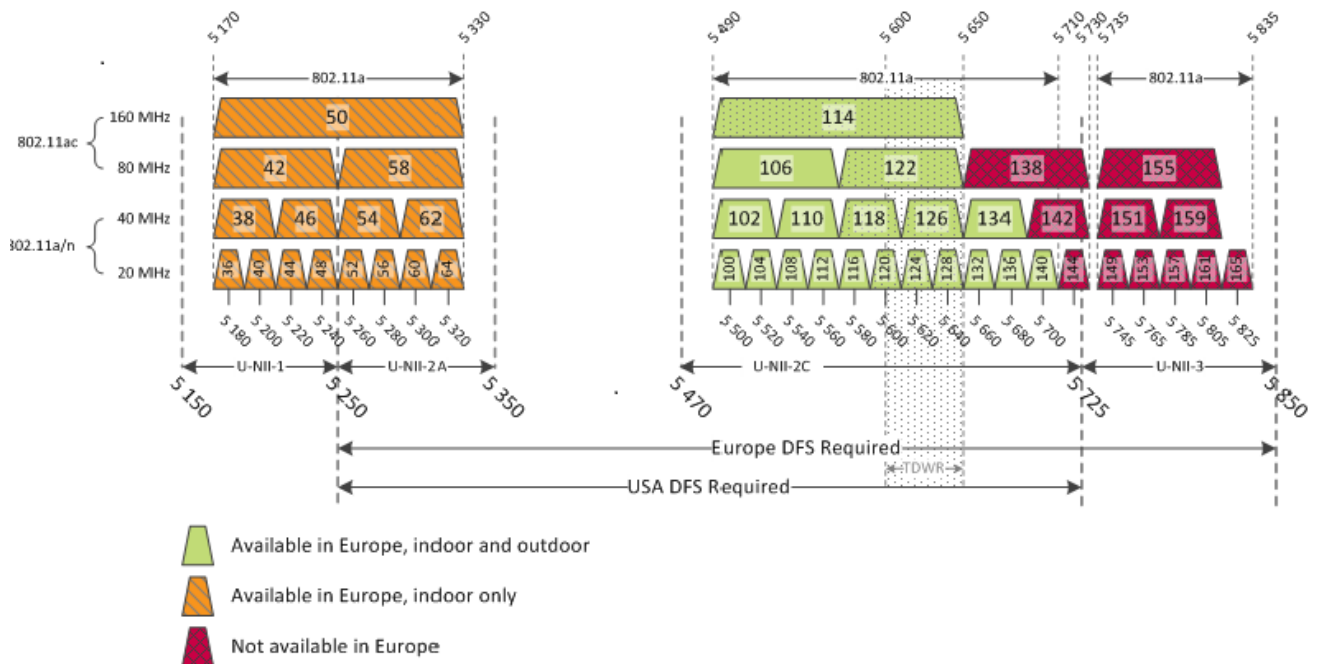
Figure 4.1: Channel arrangements for Wi-Fi in the 5 GHz band
