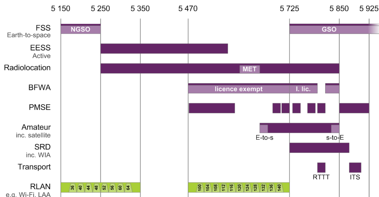
Figure 4.4 Existing UK, EU, and CEPT services in 5150-5925 MHz
