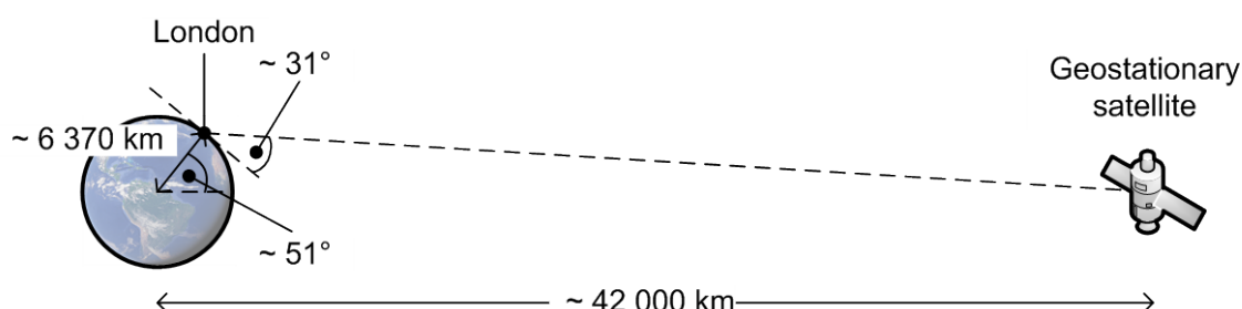
Figure A5.3: Geometry of a UK Wi-Fi/geostationary satellite coexistence scenario in 5725-5925 MHz
