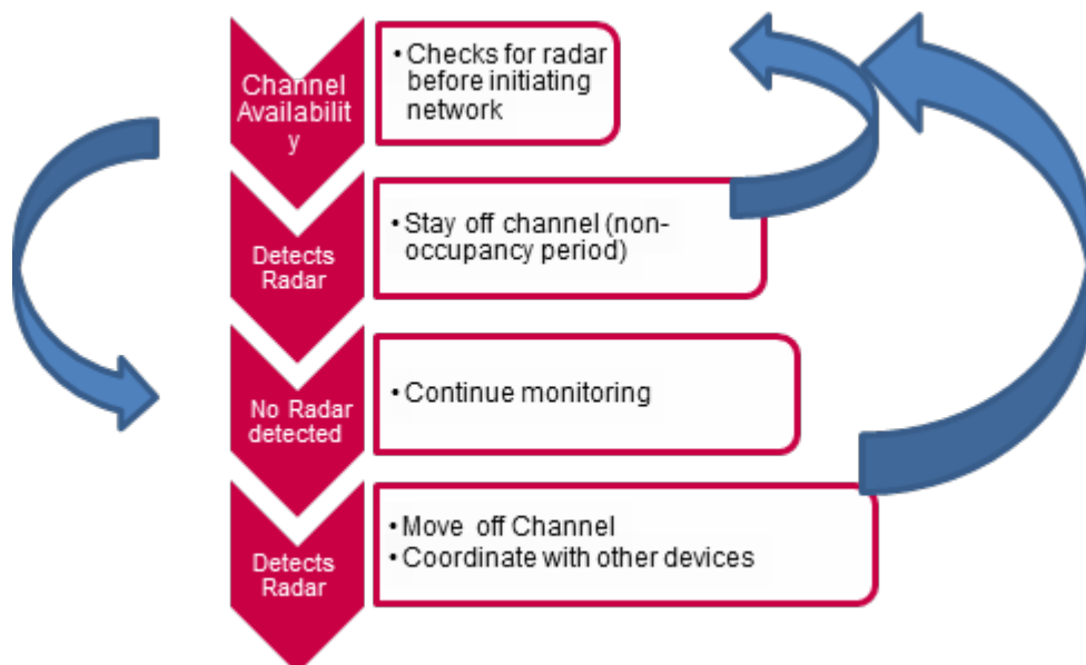
Figure 4.2: Operation of DFS
