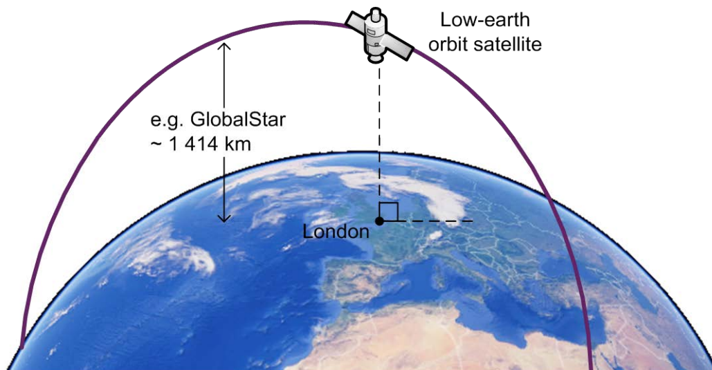
Figure A5.2: Geometry of a European Wi-Fi/low-earth orbit satellite coexistence scenario in 5150-5250 MHz
