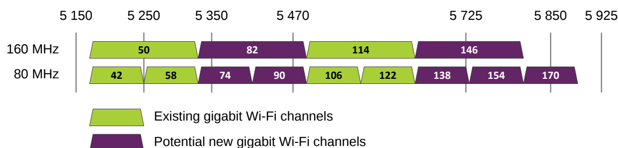
Figure A5.51: Example channelisation for Wi-Fi at 5 GHz
